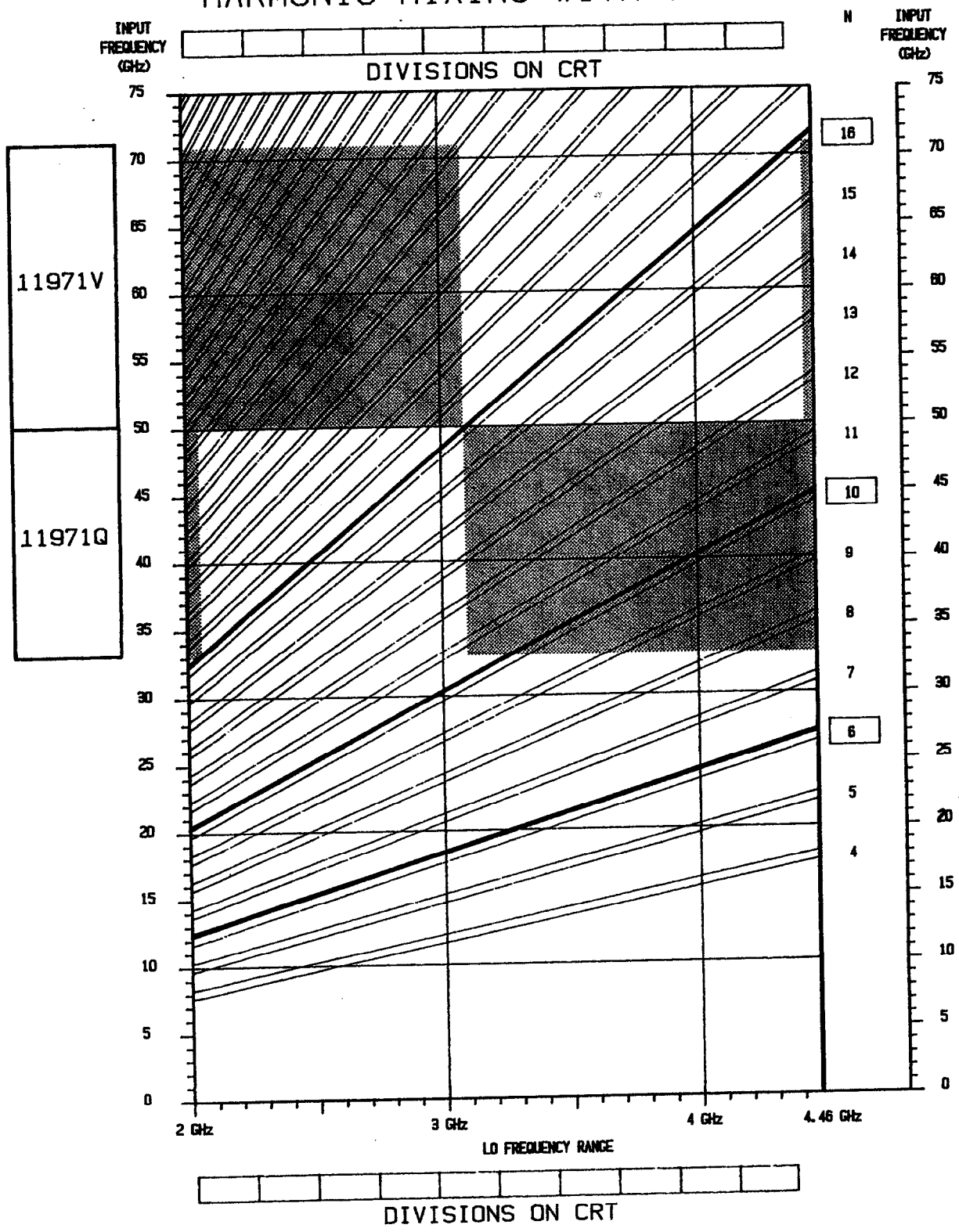
Figure 2-5. Harmonic Mixing Tuning Curves for HP 8569B
