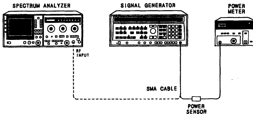
Figure 4-1. Amplitude Calibration Test Setup
