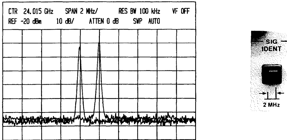
Figure 2-2. Signal Identifier
