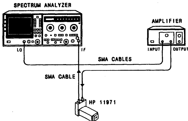
Figure 2-1. HP 11971 Mixer Connections
