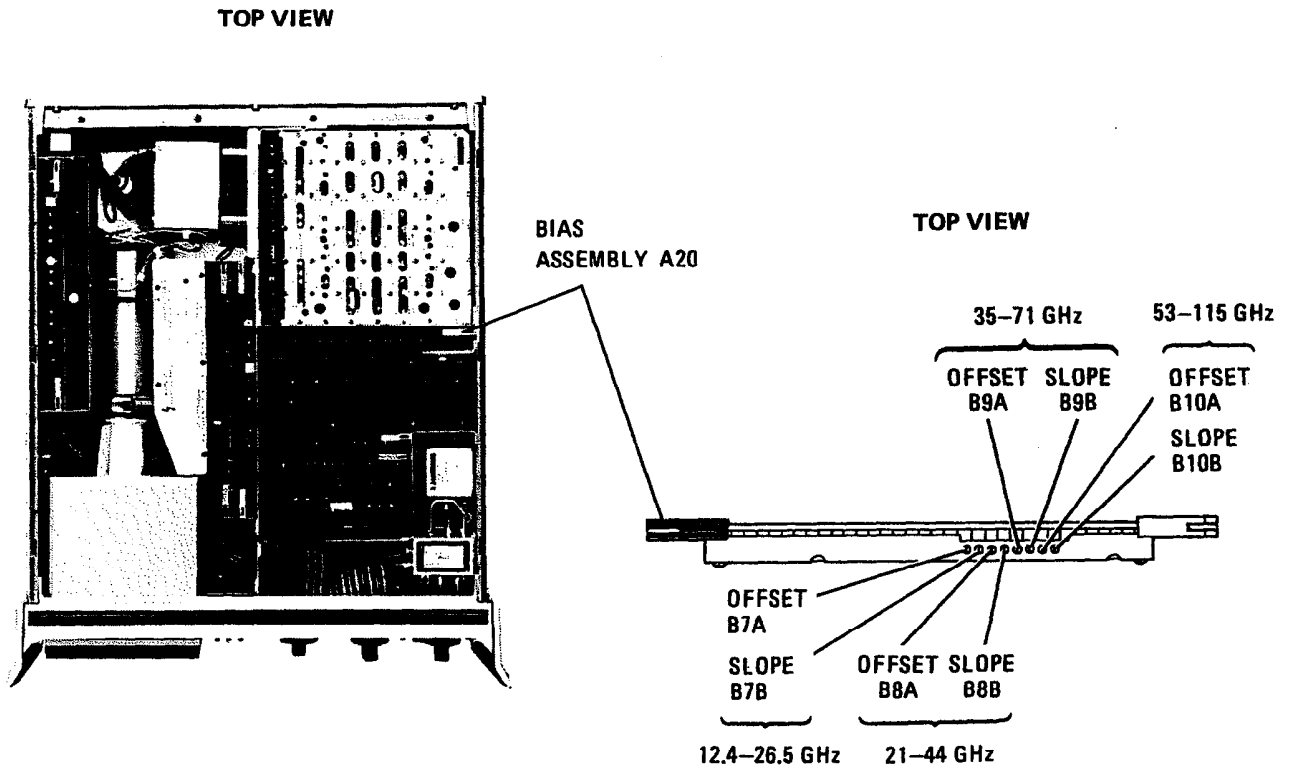
Figure 4-2. Offset and Slope Adjustment Locations
