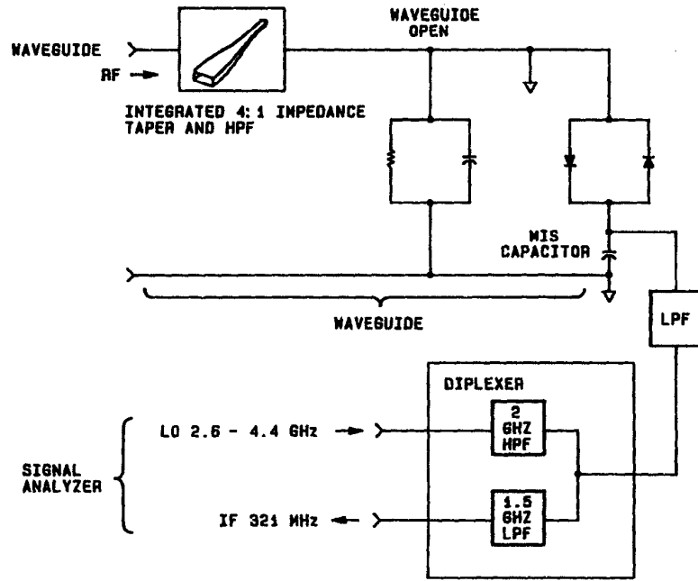
Figure 5-1. HP 11971 Series Mixer Schematic Diagram
