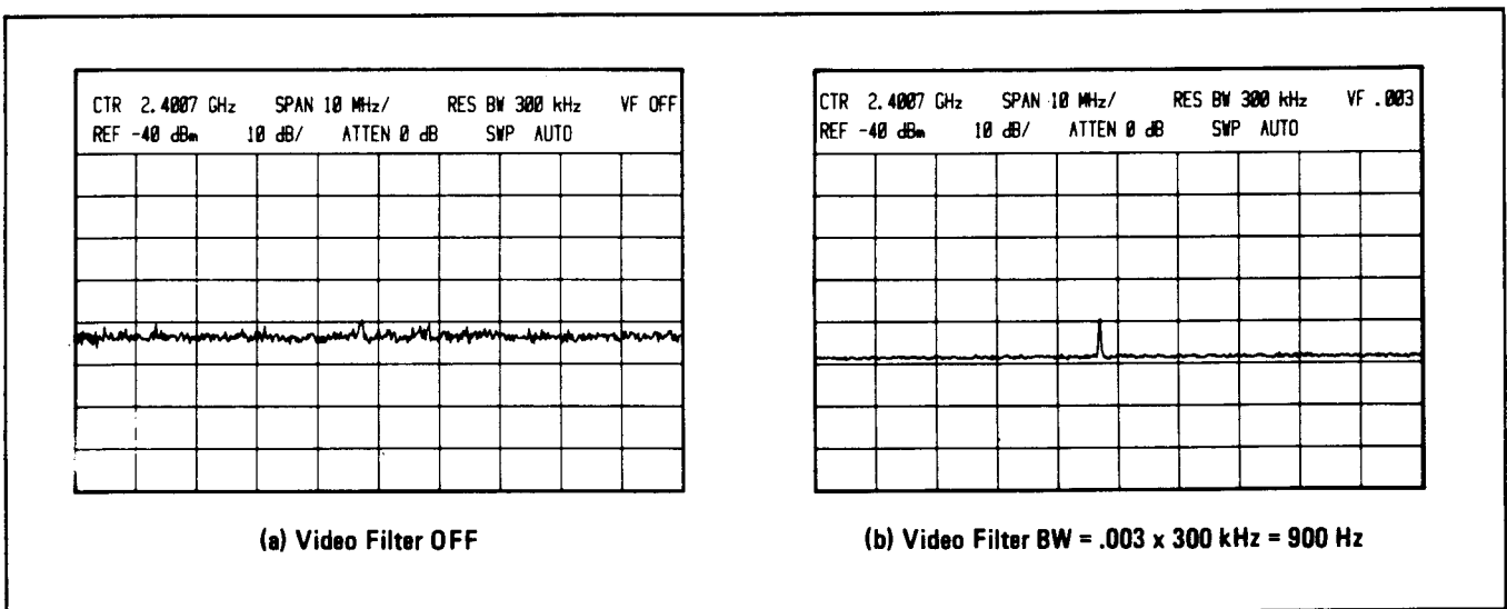
Figure 17. Video Filtering
