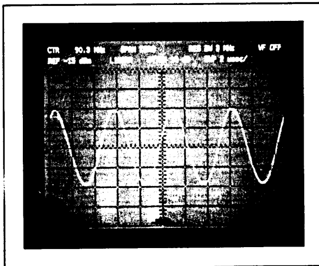
Figure 37. Demodulated AM Signal in ZERO SPAN
