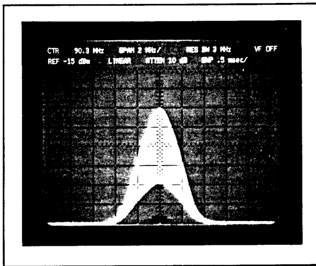
Figure 36. Linear Amplitude Display
