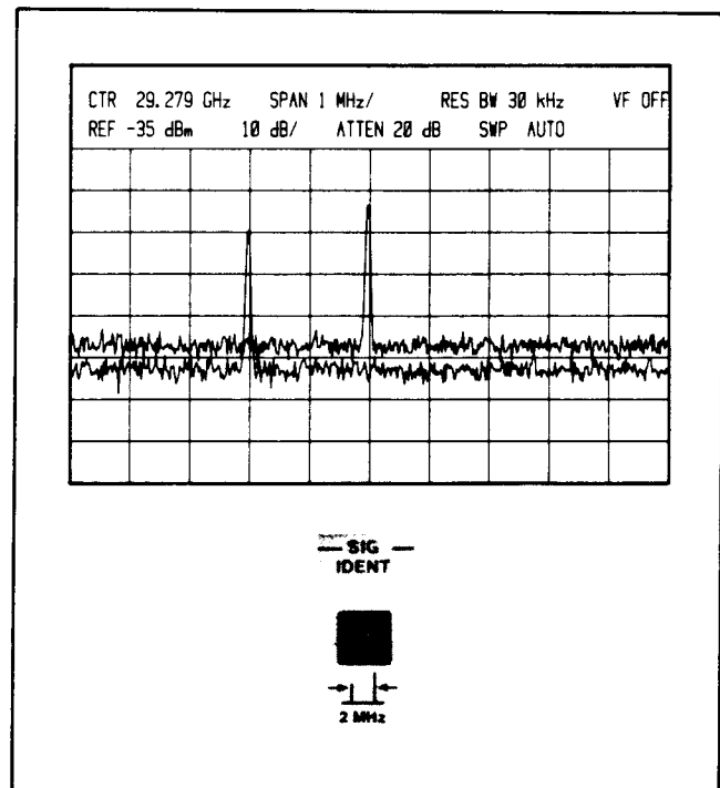
Figure 30. Signal Identifier
