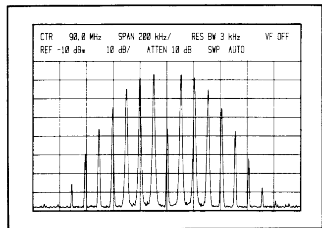
Figure 38. FM Signal
