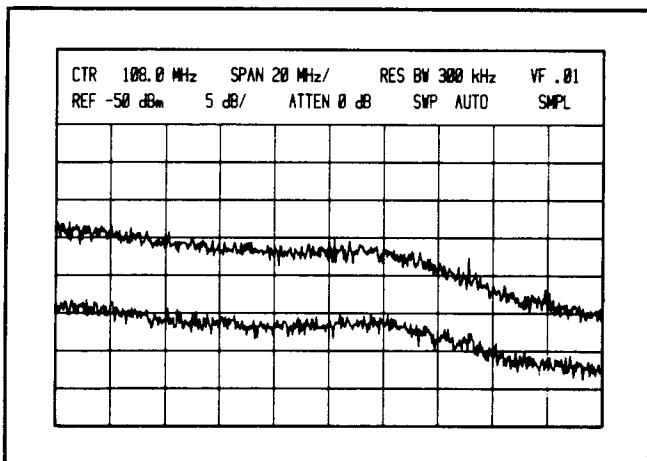
Figure 47. Y-Factor Measurement
