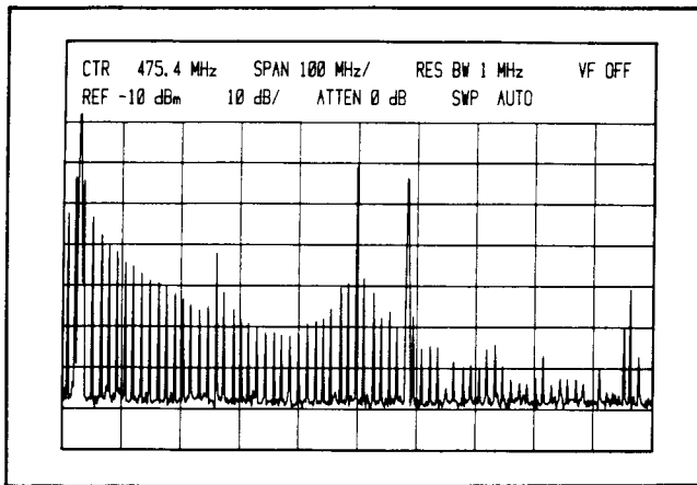
Figure 49. Radiated Interference
