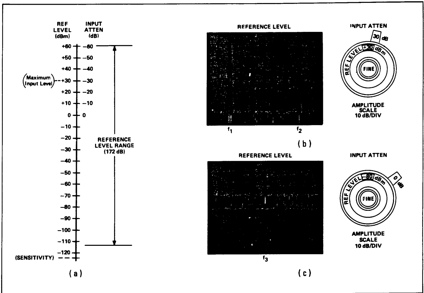
Figure 16. Reference Level
