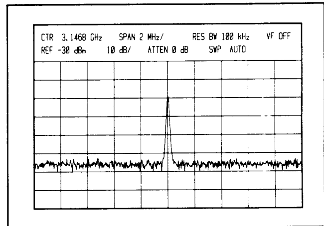
Figure 13. Analysis in PER DIV
