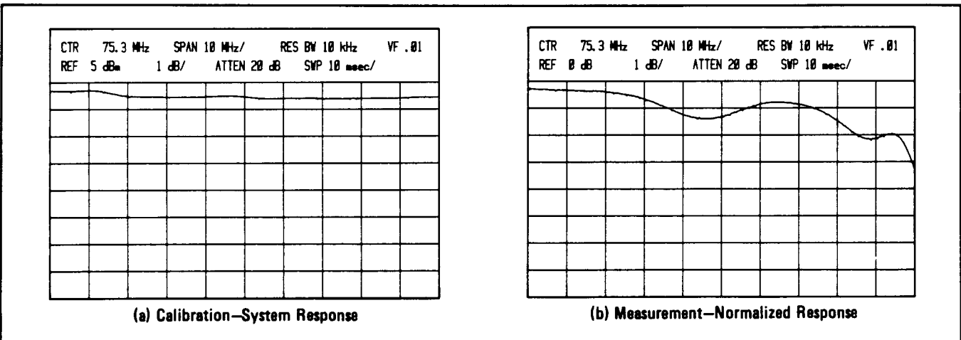
Figure 53. Normalization of Frequency Response
