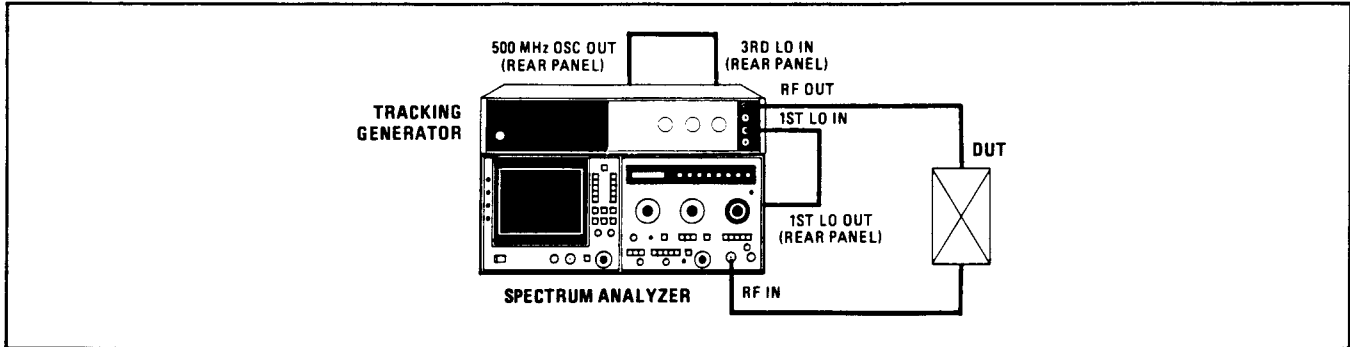
Figure 51. Swept Frequency Response Setup
