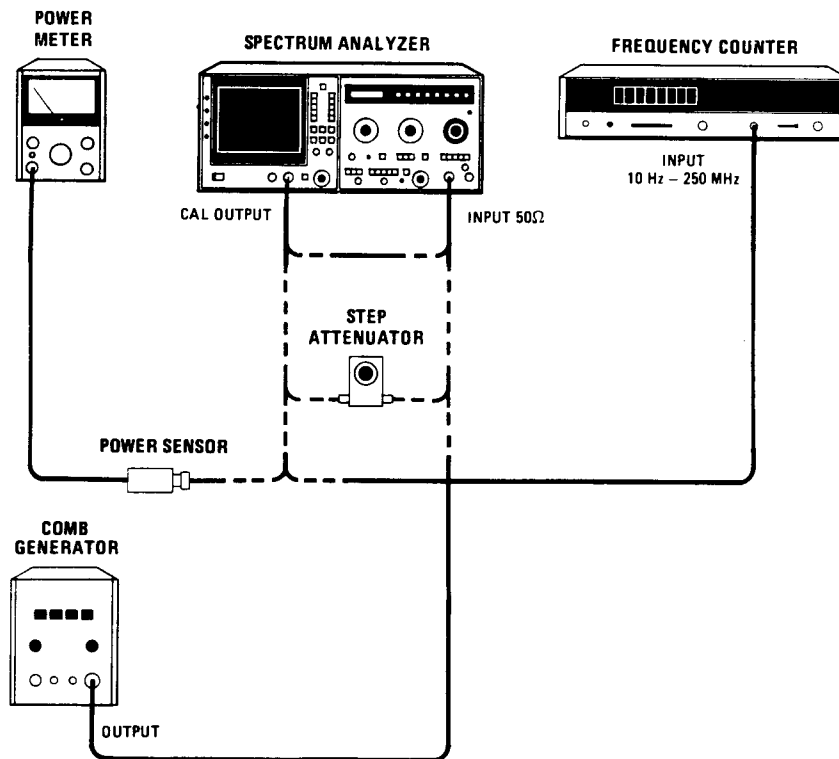
Figure 2-4. Operation Verification Test Setup
