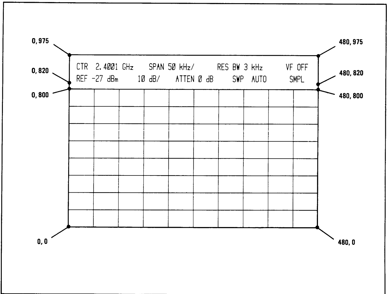
Figure 56. Display Coordinates
