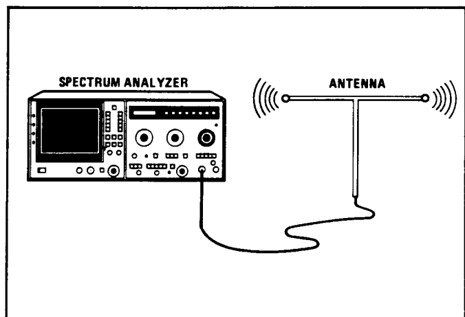
Figure 48. Field Strength Test Setup
