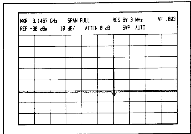
Figure 12. Identifying a Signal in FULL BAND
