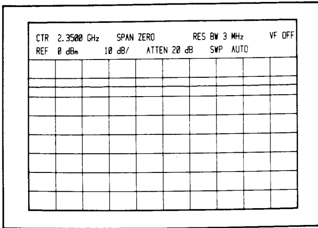
Figure 11. CW Measurement in ZERO SPAN
