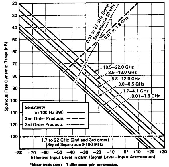
Figure 2. Optimum Dynamic Range Chart
