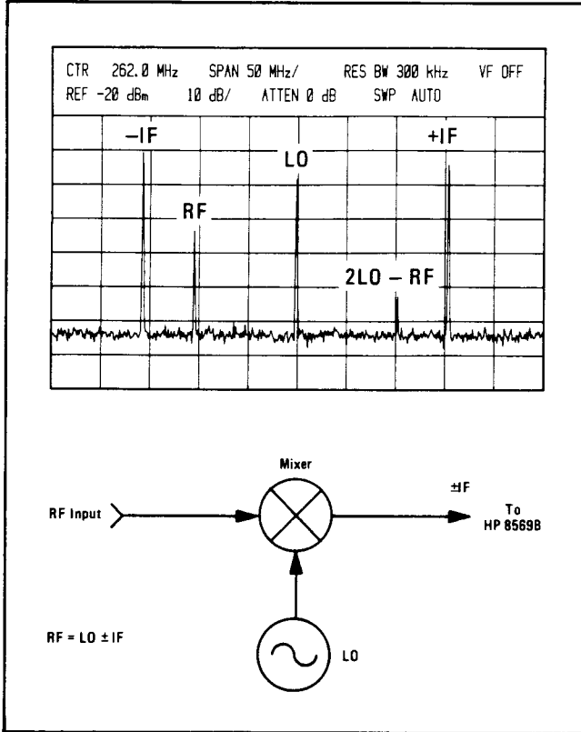
Figure 33. Mixer Measurement
