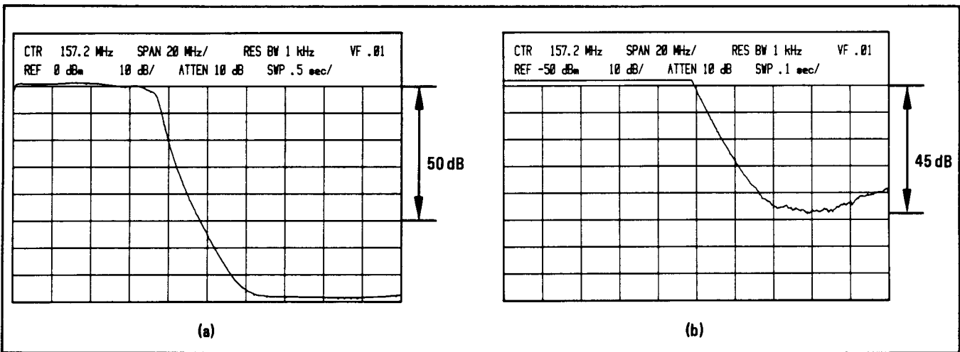
Figure 52. Low Pass Filter Measurement with 95 dB of Rejection
