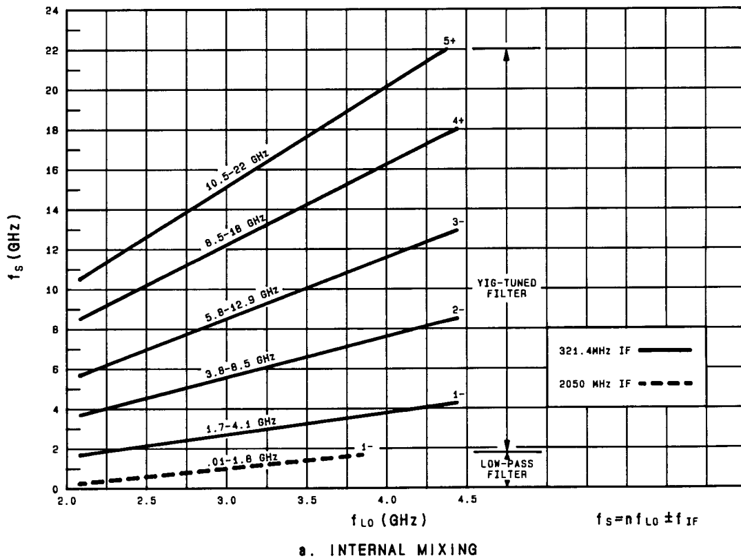
Figure B-2. HP 8569B Tuning Curves
