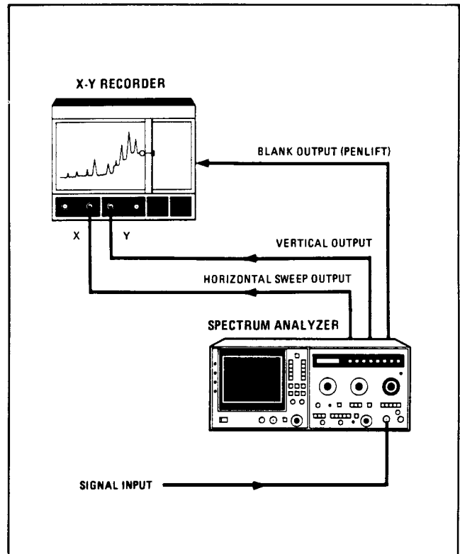
Figure 28. X-Y Recorder
