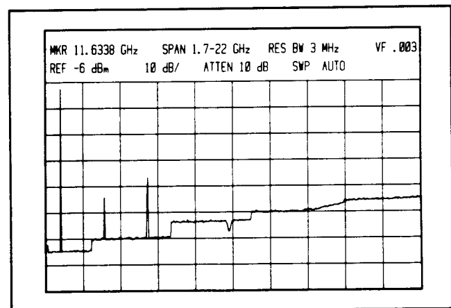
Figure 14. 1.7–22 GHz SPAN Mode
