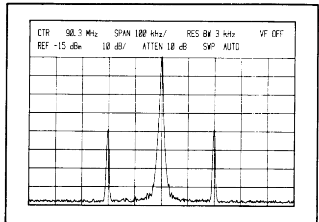
Figure 35. 2% AM
