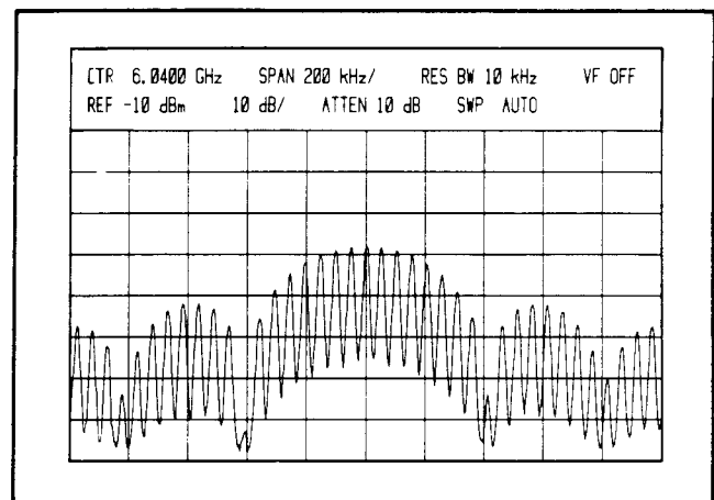
Figure 41. Line Spectrum
