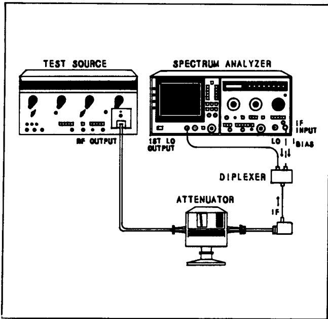
Figure 29. External Mixer Test Setup
