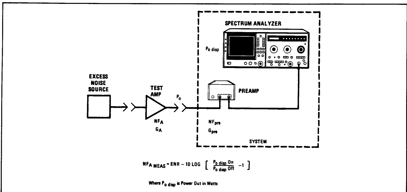
Figure 46. Measuring Noise Figure - Y Factor Technique
