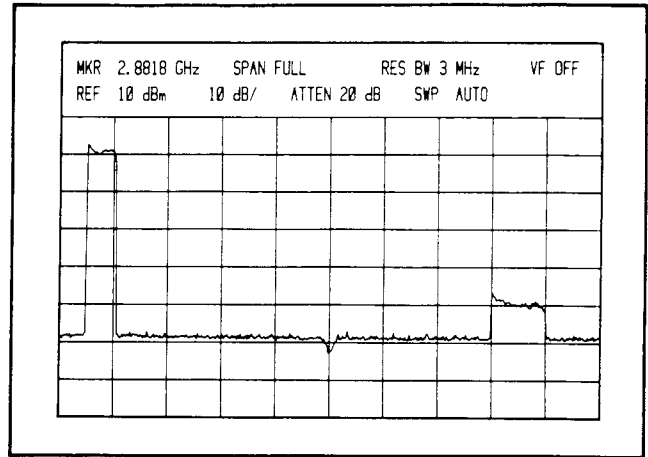
Figure 34. Oscillator Fundamental and Second Harmonic
